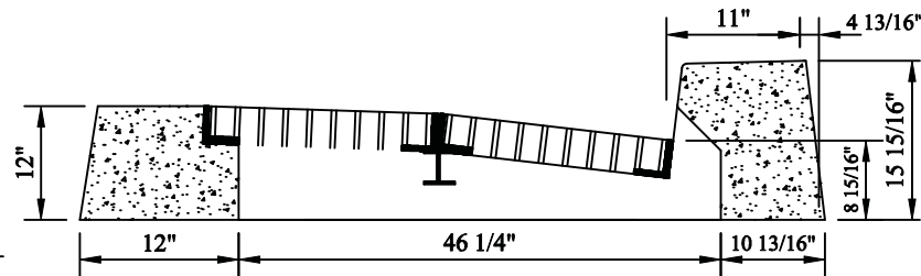
Plain Curb Type
