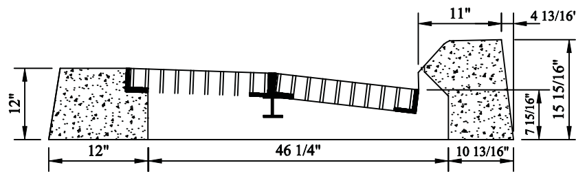
Bituminious Curb Type
